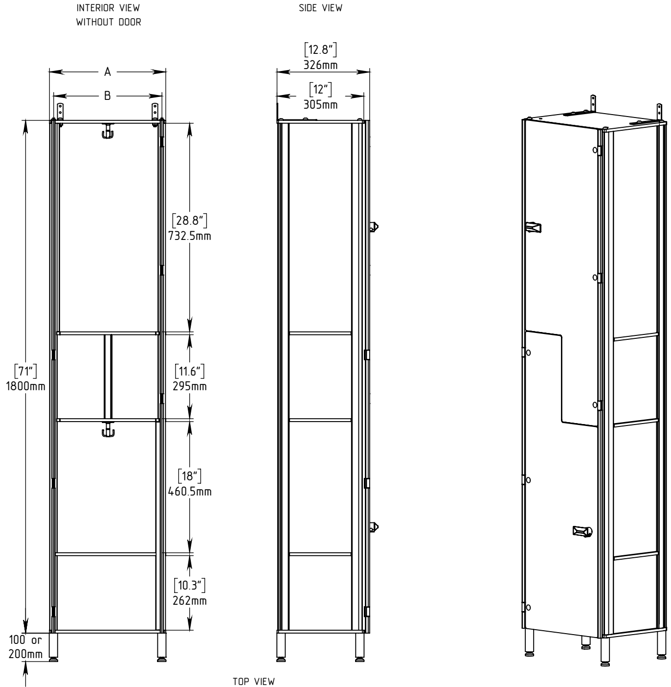
TOP VIEW
