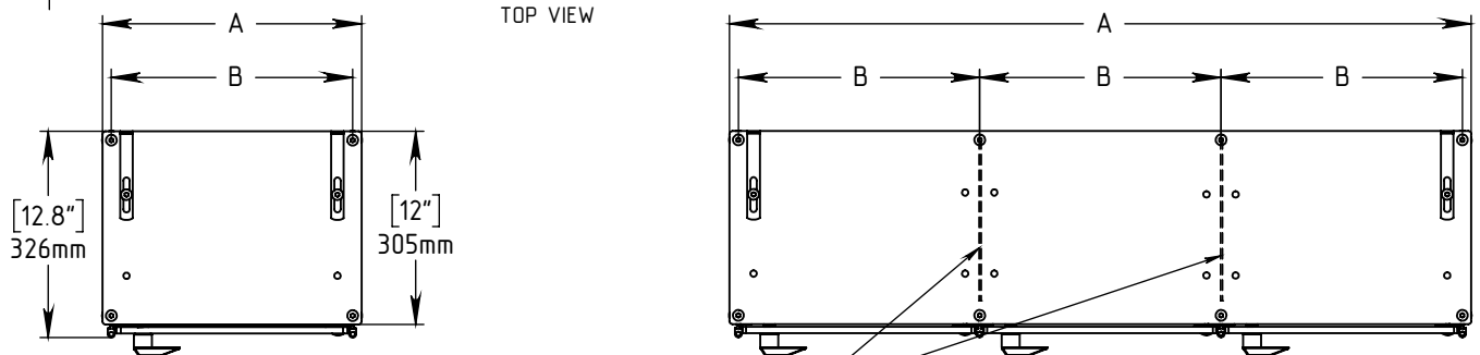
TOP VIEW
