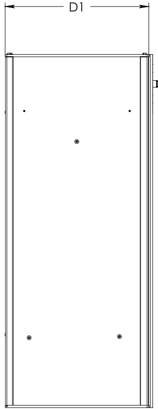
SIDE VIEW
