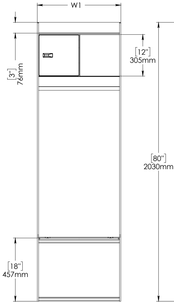
FRONT VIEW
