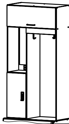
ISOMETRIC VIEW GIRLS/WOMENS DESIGN
