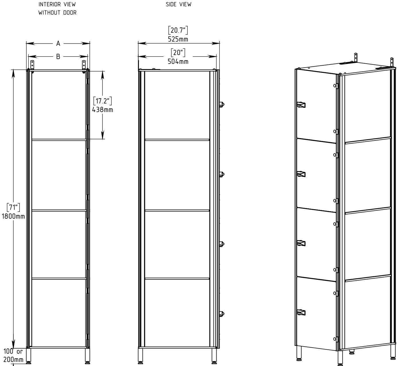
TOP VIEW
